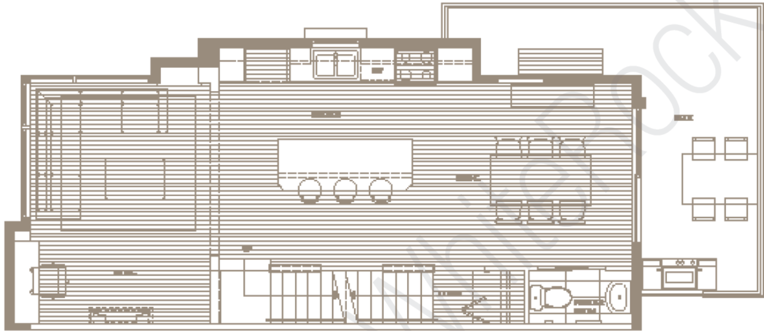
FLOOR 2
