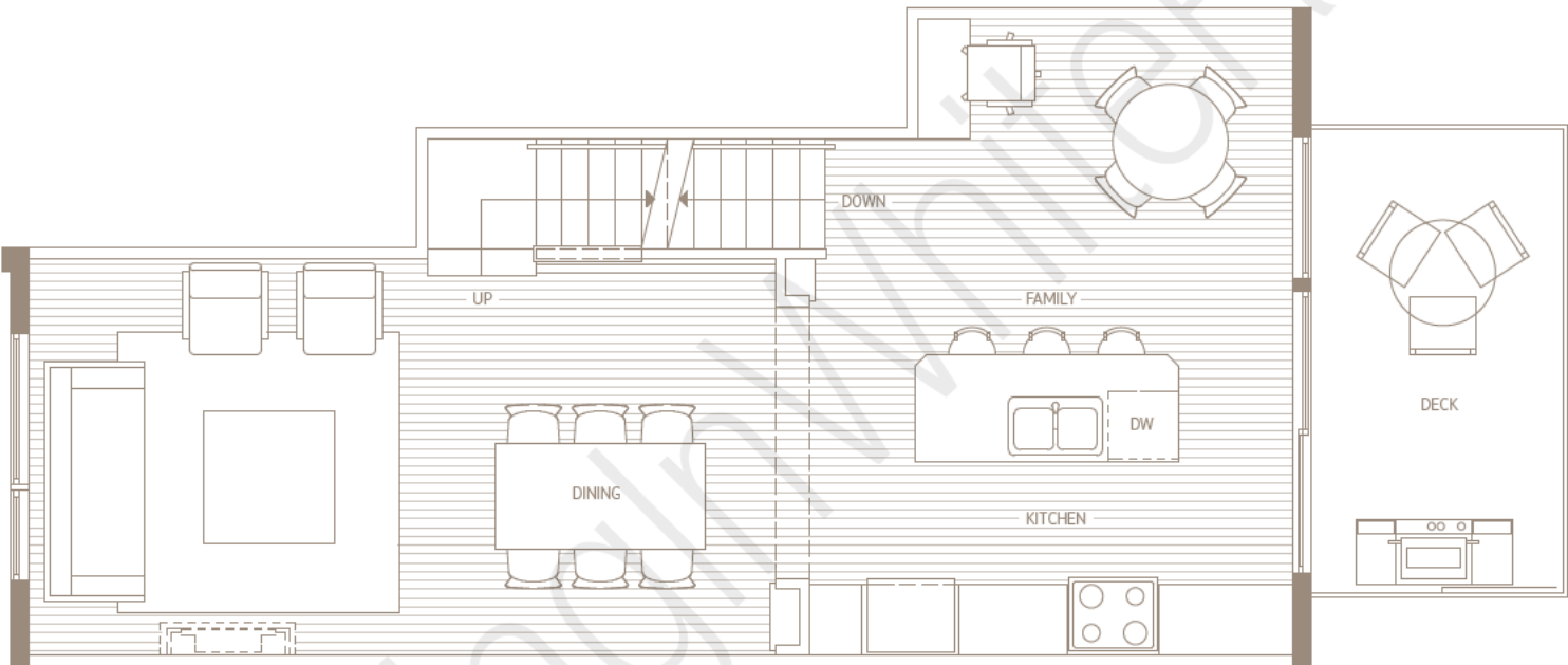
FLOOR 2
