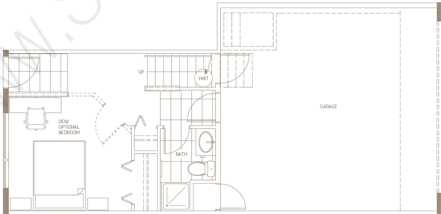
FLOOR 1
